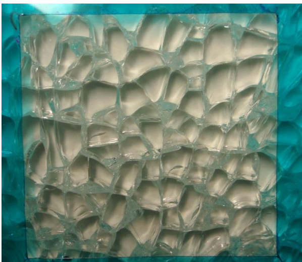
Figure 5. Fragmentation of specimen 3.
