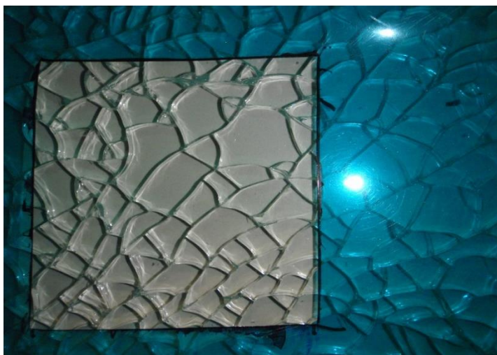
Figure 5. Fragmentation of specimen 3.
